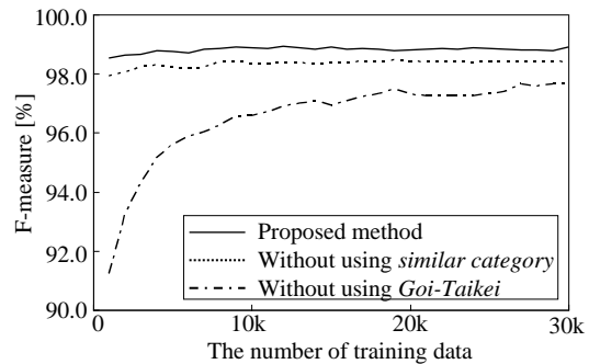
Figure 7: The effects of using similar categories and Goi-Taikei
