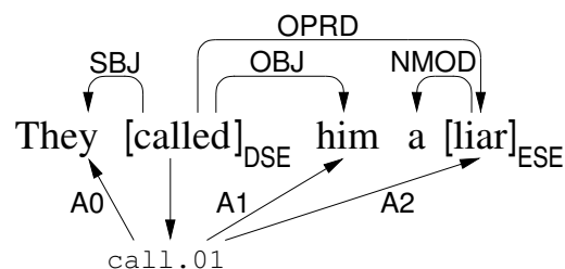
Figure 1: Syntactic and shallow semantic structure.
