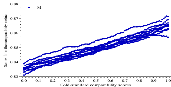
Figure 1: Evolution of M wrt gold-standard on the corpus group G_c (x-axis: gold-standard comparability scores, y-axis: M scores)
