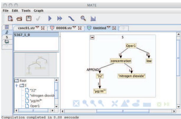
Figure 5: Graph Editor
